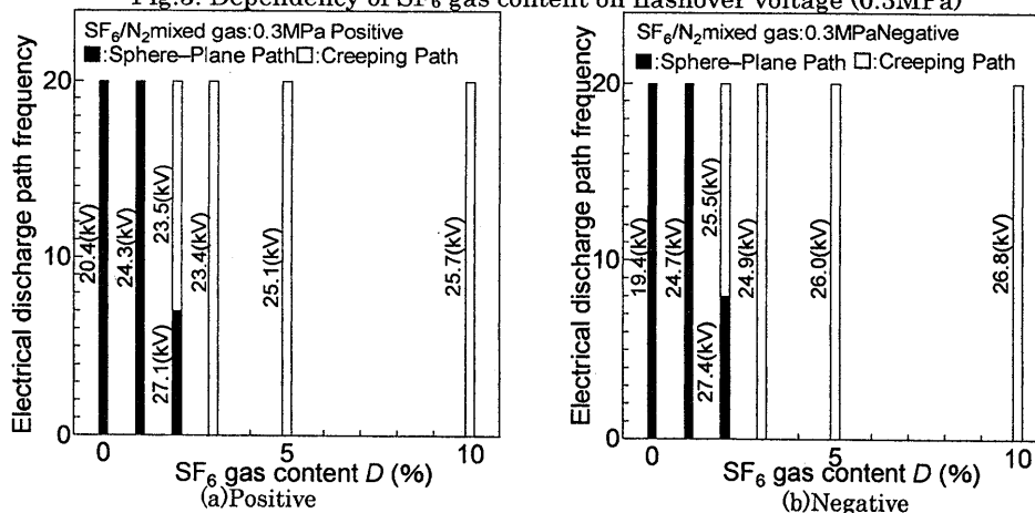
図4 各放電経路回数 - 混合率特性 Fig.4. Dependency of \text{SF}_6 gas content on electrical discharge path frequency
